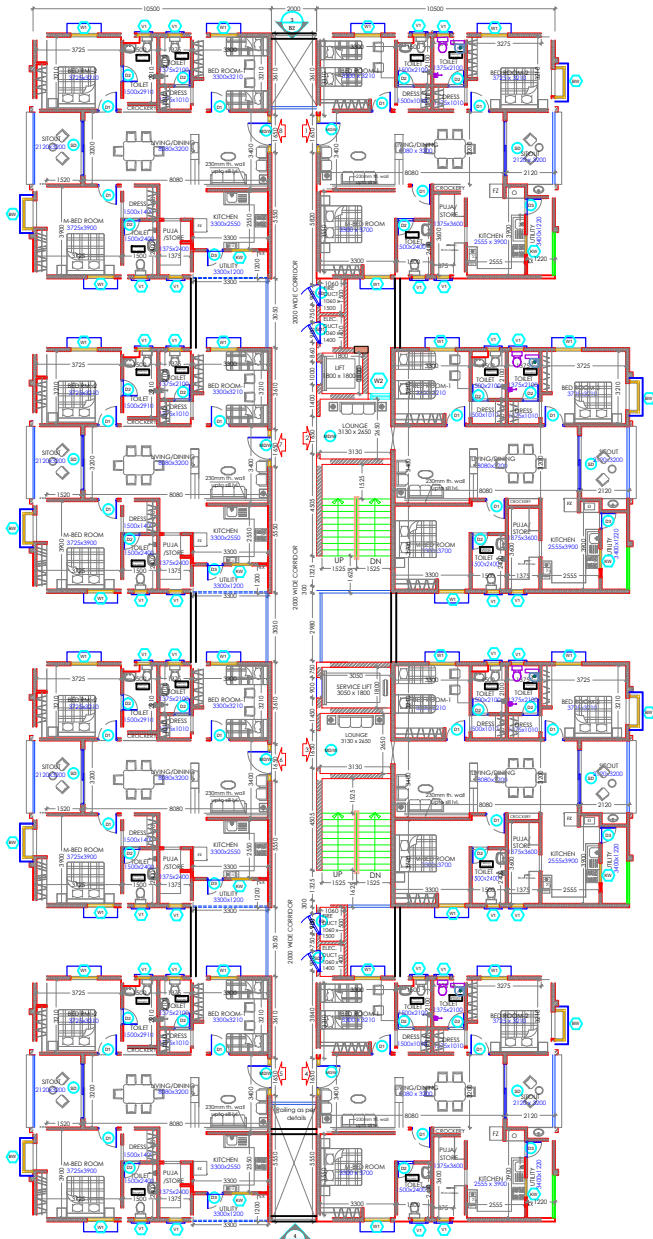
11 1ST TO 11TH FLOOR PLAN Scale: 1/100
