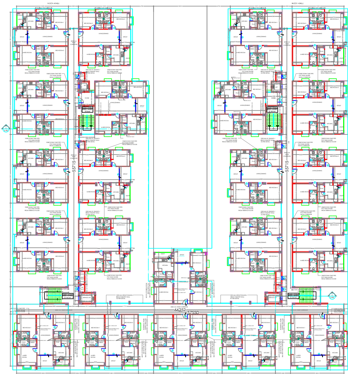
3rd, 6th & 9th FLOOR PLAN Scale: 1:100
