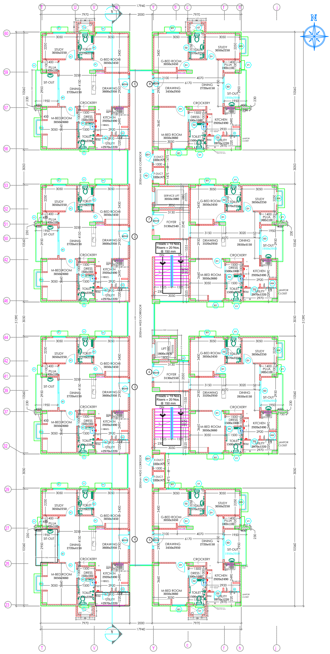
TYPICAL FLOOR PLAN BLOCK - B04
